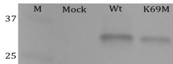
Figure 1: Wild type (Wt) or kinase dead (K69M) PIM-3 was expressed with BAD transiently in 293 cells. Following cell lysis, a Western was performed with appropriate antibodies to detect total PIM-3 protein.
