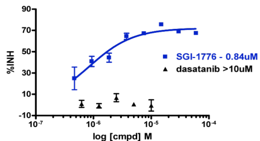
Figure 4: A phosphorylation assay was performed in the presence of SGI-1776, a PIM-3 inhibitor, and dasatanib, a compound that is not expected to inhibit PIM-3. % inhibition data were plotted to determine EC 50 s.
